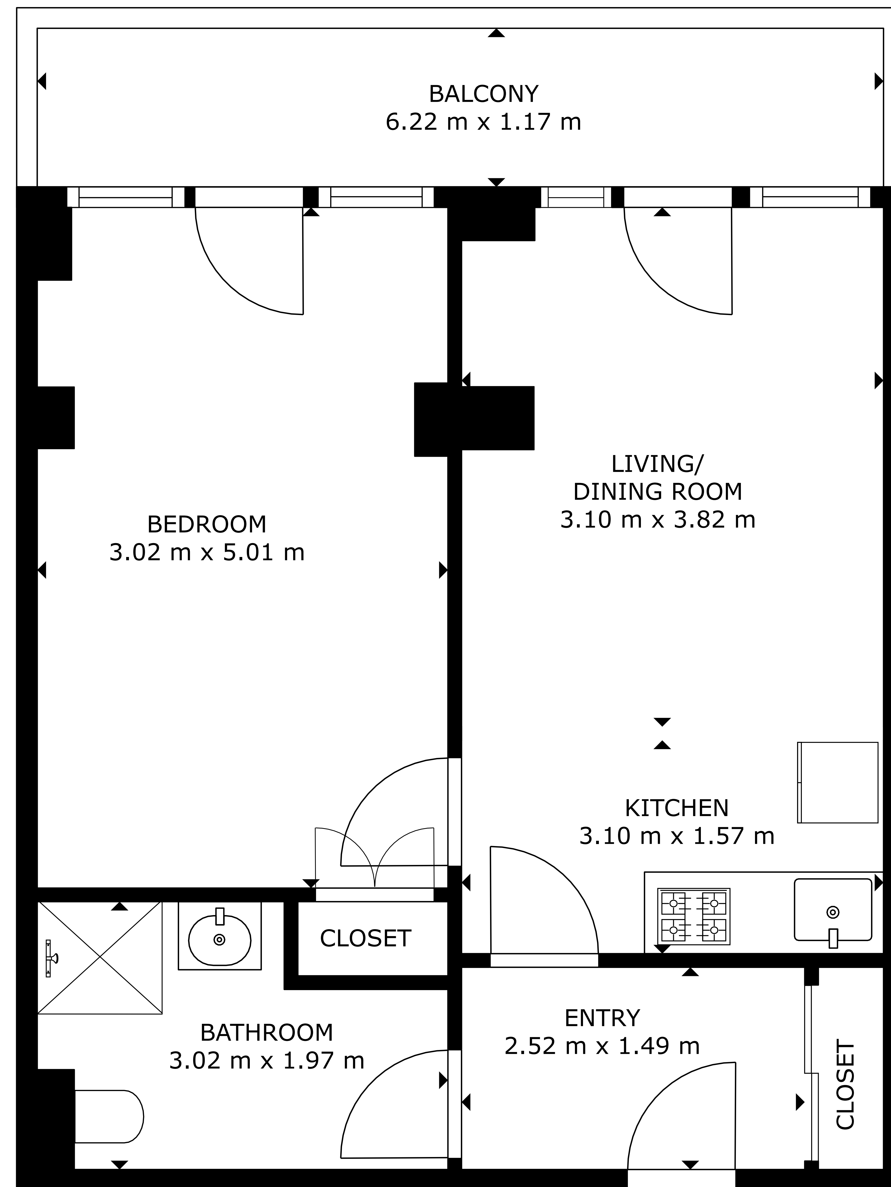
FLOOR PLAN
